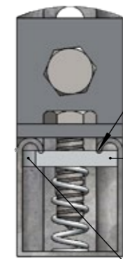
JOINING UNISTRUT'S
